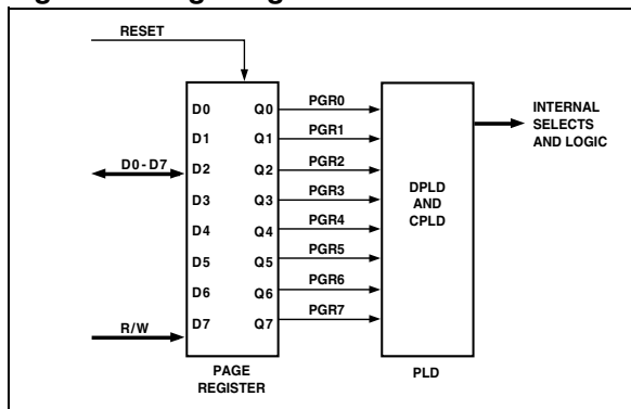
Figure 12. Page Register
